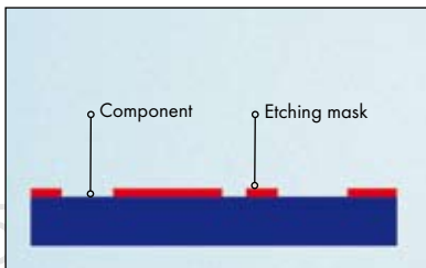
Component with etching mask before plasma treatment
